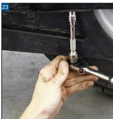
23 Install the lower belt guard's three mounting screws. That's it! You're all set for wobble-free highway riding.
