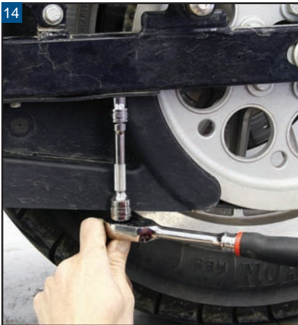
14 The rear True-Track installation begins with the removal of the three mounting screws.
